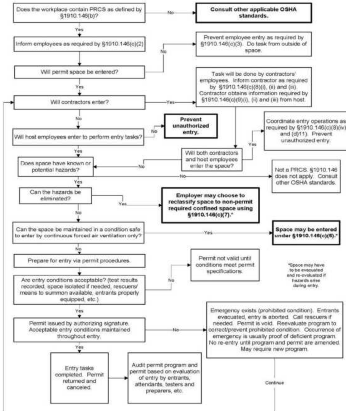
FIGURE 34-1 Confined Space Identification Flow Chart
