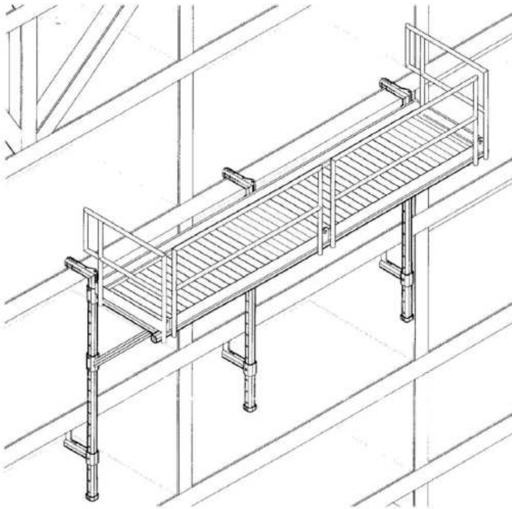
FIGURE 22-1 Hanging Scaffold
